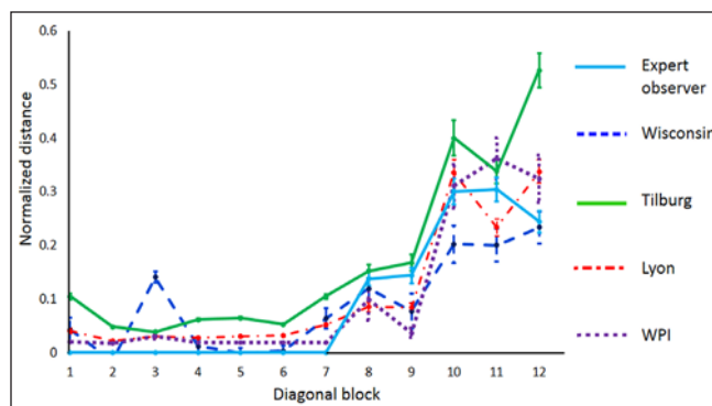
Figure 4. Normalized image pair distances for the dataset of texture images (Diagonal blocks 1-3 same sheet, 4-6 same package, 7-9 same manufacturing standard and, 10-12 diverse samples).
